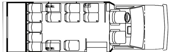
AC 23 159" Wheelbase
