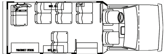
AC 21 159" Wheelbase
